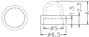
Screw Bonnet
