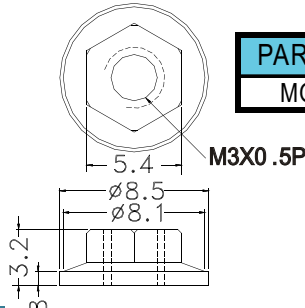
Flange Nut (Nylon)
